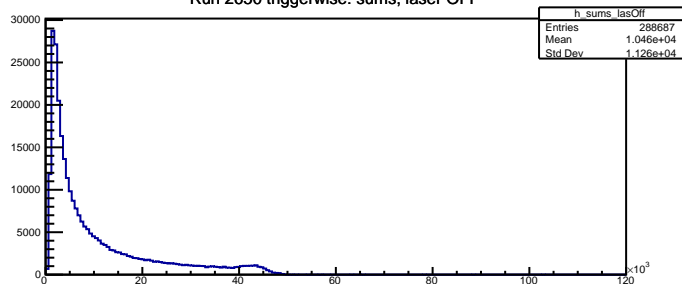
Run 2650 triggerwise: sums, laser OFF
