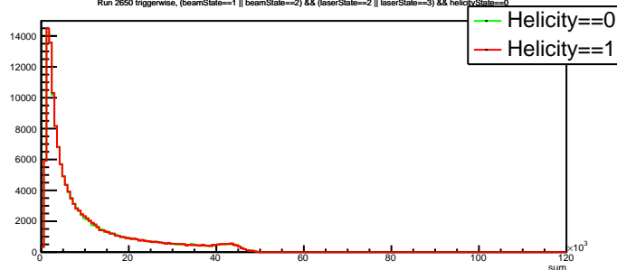
Run 2650 triggerwise, (beamState==1 || beamState==2) &amp;&amp; (laserState==2 || laserState==3) &amp;&amp; helicityState==0
