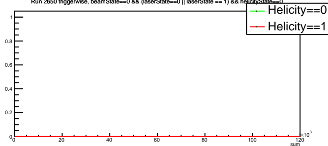
Run 2650 triggerwise, beamState==0 &amp;&amp; (laserState==0 || laserState == 1) &amp;&amp; helicityState==0
