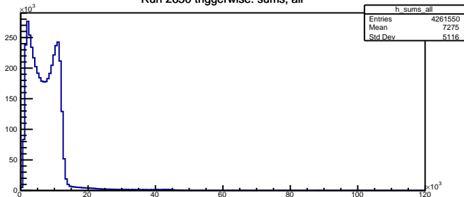
Run 2650 triggerwise: sums, all
