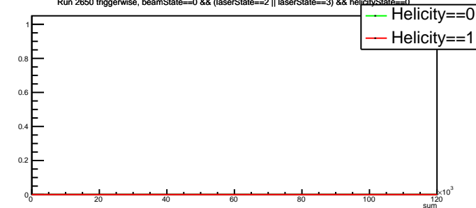
Run 2650 triggerwise, beamState==0 &amp;&amp; (laserState==2 || laserState==3) &amp;&amp; helicityState==0
