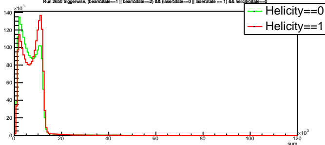
Run 2650 triggerwise, (beamState==1 || beamState==2) &amp;&amp; (laserState==0 || laserState == 1) &amp;&amp; helicityState==0
