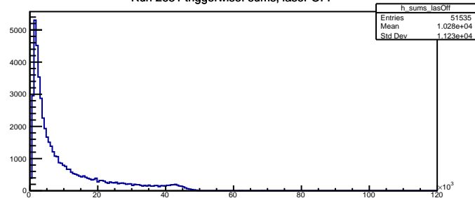
Run 2651 triggerwise: sums, laser OFF
