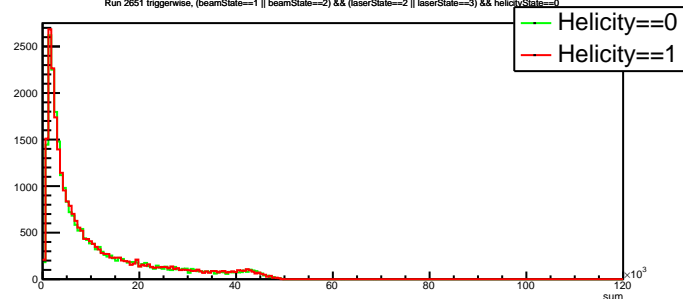
Run 2651 triggerwise, (beamState==1 || beamState==2) &amp;&amp; (laserState==2 || laserState==3) &amp;&amp; helicityState==0
