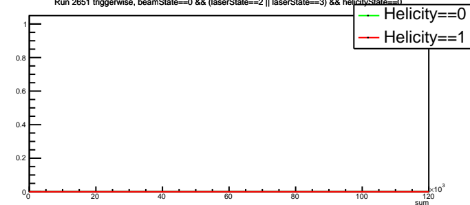
Run 2651 triggerwise, beamState==0 &amp;&amp; (laserState==2 || laserState==3) &amp;&amp; helicityState==0
