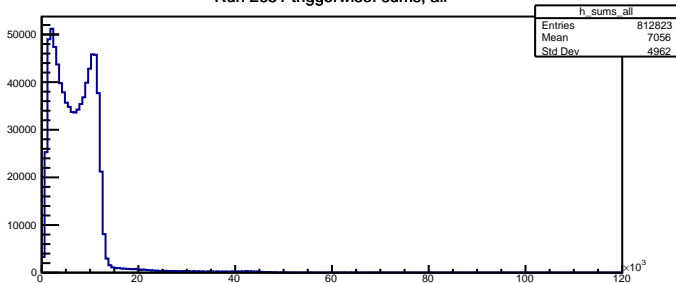
Run 2651 triggerwise: sums, all
