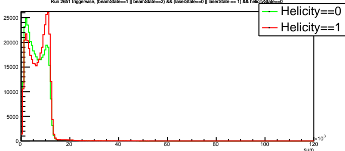
Run 2651 triggerwise, (beamState==1 || beamState==2) &amp;&amp; (laserState==0 || laserState == 1) &amp;&amp; helicityState==0
