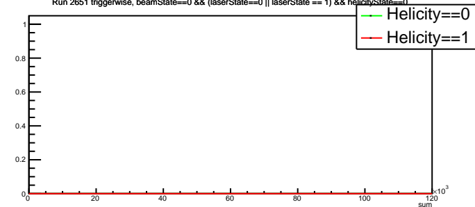
Run 2651 triggerwise, beamState==0 &amp;&amp; (laserState==0 || laserState == 1) &amp;&amp; helicityState==0
