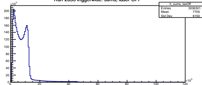
Run 2655 triggerwise: sums, laser OFF
