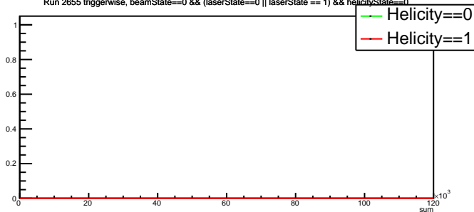
Run 2655 triggerwise, beamState==0 &amp;&amp; (laserState==0 || laserState == 1) &amp;&amp; helicityState==0
