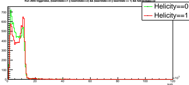
Run 2655 triggerwise, (beamState==1 || beamState==2) &amp;&amp; (laserState==0 || laserState == 1) &amp;&amp; helicityState==0
