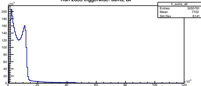
Run 2655 triggerwise: sums, all
