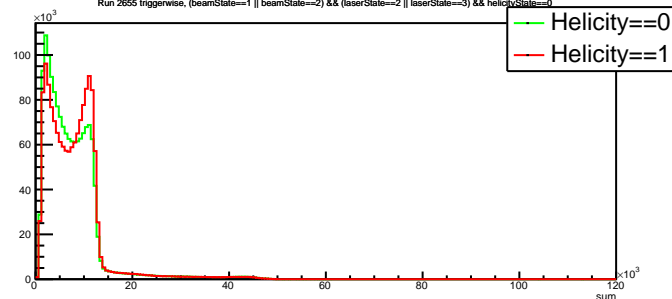
Run 2655 triggerwise, (beamState==1 || beamState==2) &amp;&amp; (laserState==2 || laserState==3) &amp;&amp; helicityState==0
