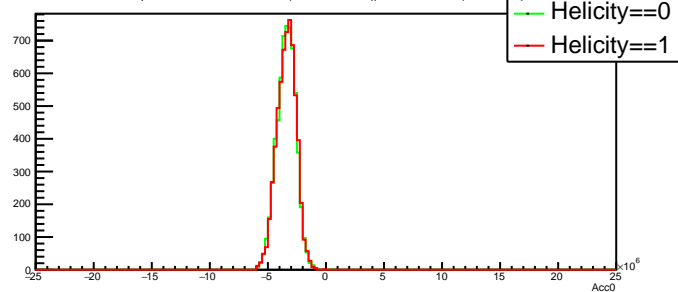
Run 2656 mpwise, beamState==0 &amp;&amp; (laserState==0 || laserState == 1) &amp;&amp; helicityState==0
