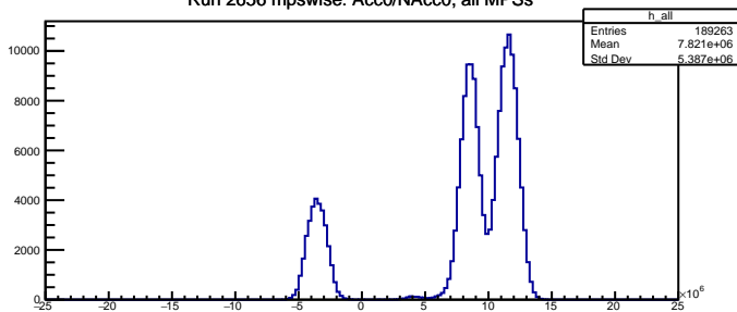
Run 2656 mpwise: Acc0/NAcc0, all MPSs
