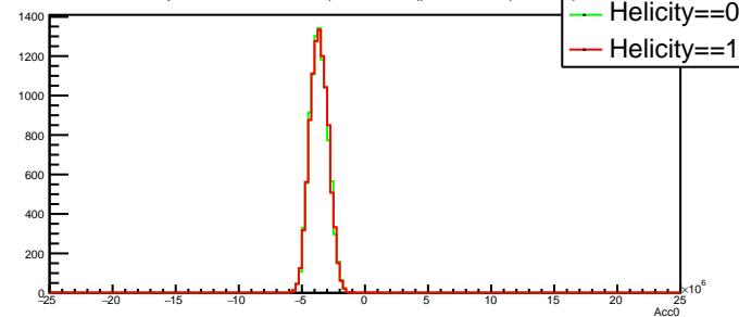
Run 2656 mpwise, beamState==0 &amp;&amp; (laserState==2 || laserState==3) &amp;&amp; helicityState==0
