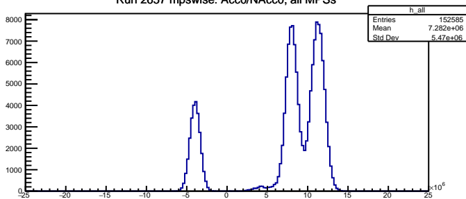
Run 2657 mpwise: Acc0/NAcc0, all MPSs
