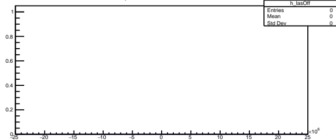
Run 2658 mpwise: Acc0/NAcc0, laser OFF
