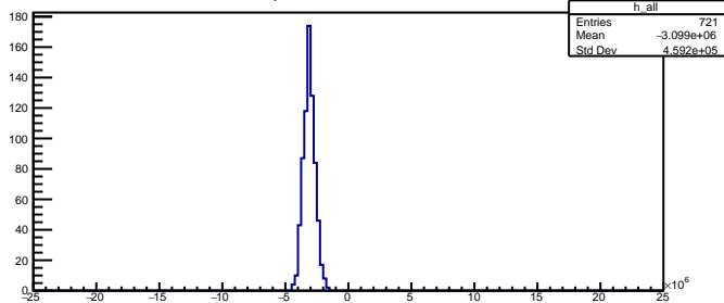
Run 2658 mpwise: Acc0/NAcc0, all MPSs
