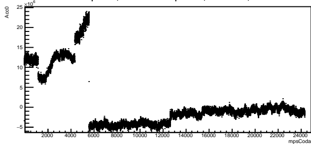
Run 2659 mpwise, Acc0/NAcc0:mpsCoda, beam OFF, laser OFF
