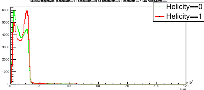
Run 2660 triggerwise, (beamState==1 || beamState==2) &amp;&amp; (laserState==0 || laserState == 1) &amp;&amp; helicityState==0
