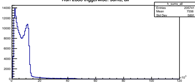
Run 2660 triggerwise: sums, all
