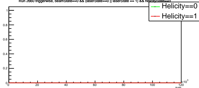
Run 2660 triggerwise, beamState==0 &amp;&amp; (laserState==0 || laserState == 1) &amp;&amp; helicityState==0
