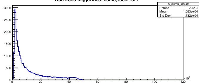
Run 2660 triggerwise: sums, laser OFF
