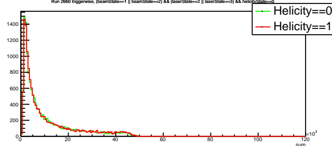
Run 2660 triggerwise, (beamState==1 || beamState==2) &amp;&amp; (laserState==2 || laserState==3) &amp;&amp; helicityState==0
