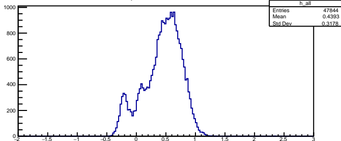
Run 3843 mpwise: Acc0/NAcc0, all MPSS
