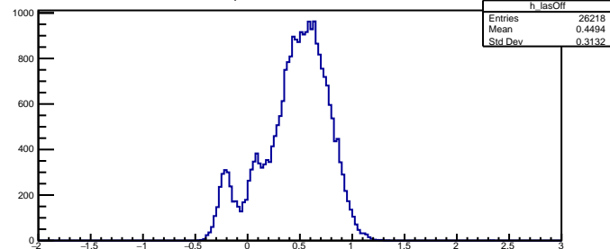
Run 3843 mpwise: Acc0/NAcc0, laser OFF
