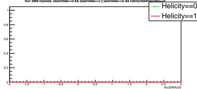
Run 3968 mpwise, beamState==0 &amp;&amp; (laserState==2 || laserState==3) &amp;&amp; helicityStateReported==0
