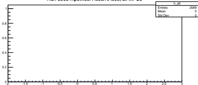
Run 3968 mpwise: Acc0/NAcc0, all MPSs
