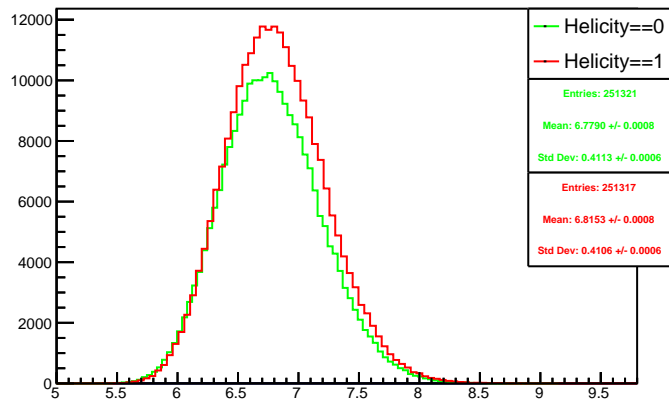
Run 4342 mpwise, acc0: Beam ON, Laser OFF
