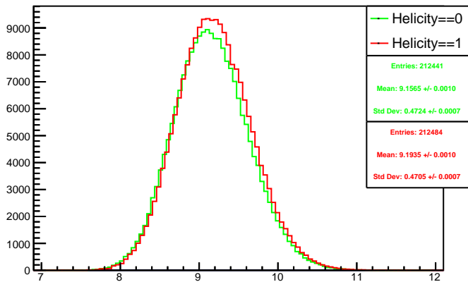
Run 4342 mpwise, acc0: Beam ON, Laser ON
