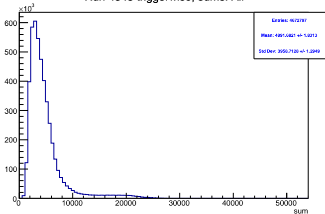
Run 4343 triggerwise, sums: All
