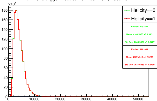
Run 4343 triggerwise, sums: Beam ON, Laser OFF
