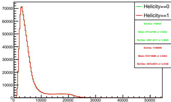
Run 4344 triggerwise, sums: Beam ON, Laser ON
