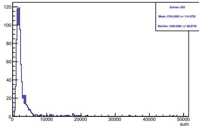
Run 4344 triggerwise, sums: Beam ON, Laser OFF
