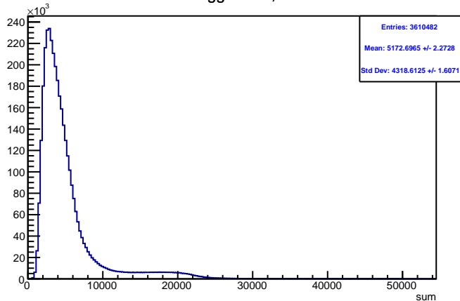
Run 4344 triggerwise, sums: All
