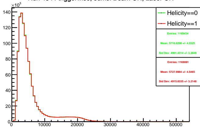
Run 4344 triggerwise, sums: Beam ON, Laser ON
