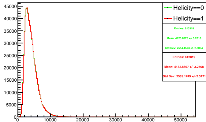
Run 4344 triggerwise, sums: Beam ON, Laser OFF
