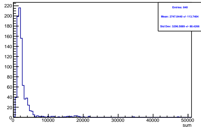
Run 4344 triggerwise, sums: Beam ON, Laser OFF
