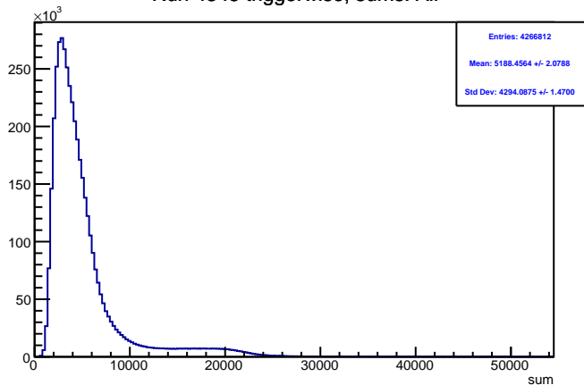
Run 4345 triggerwise, sums: All
