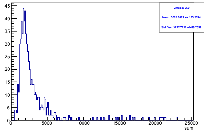
Run 4345 triggerwise, sums: Beam ON, Laser OFF
