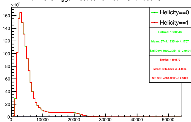
Run 4345 triggerwise, sums: Beam ON, Laser ON
