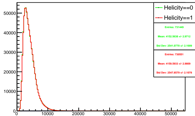
Run 4345 triggerwise, sums: Beam ON, Laser OFF
