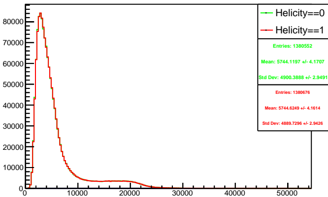
Run 4345 triggerwise, sums: Beam ON, Laser ON
