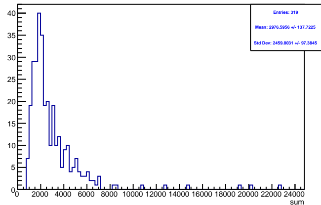
Run 4346 triggerwise, sums: Beam ON, Laser OFF
