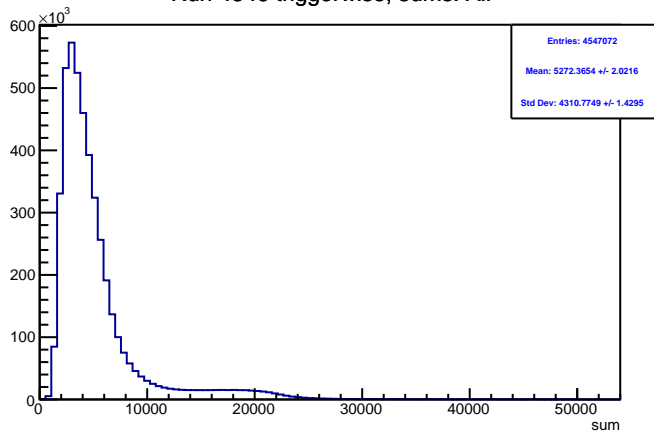
Run 4346 triggerwise, sums: All
