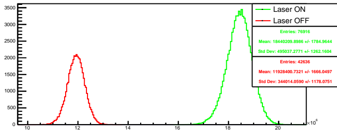
Run 4348 quartetwise, posH4: Beam ON
