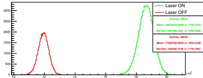
Run 4348 quartetwise, negH4: Beam ON
