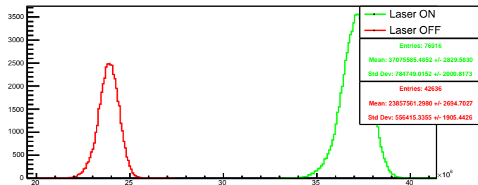
Run 4348 quartetwise, summ4: Beam ON
