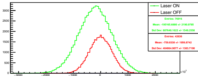
Run 4348 quartetwise, diff4: Beam ON
