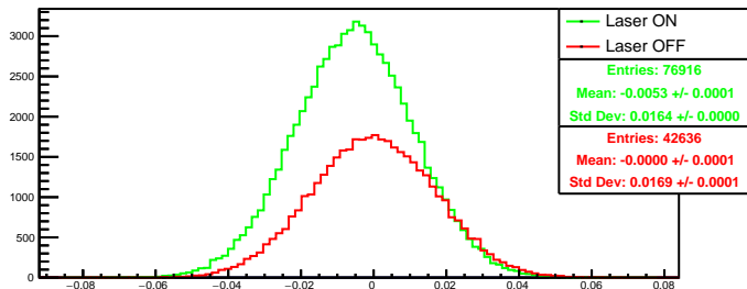
Run 4348 quartetwise, asym4: Beam ON
