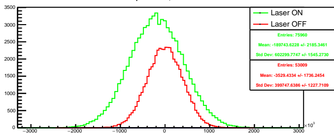
Run 4349 quartetwise, diff4: Beam ON
