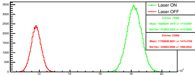
Run 4349 quartetwise, posH4: Beam ON
