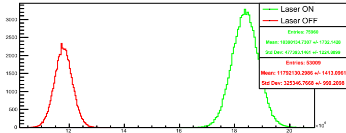
Run 4349 quartetwise, negH4: Beam ON
