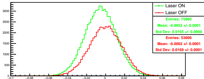
Run 4349 quartetwise, asym4: Beam ON
