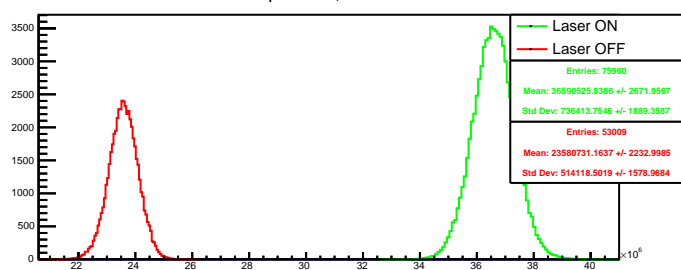
Run 4349 quartetwise, summ4: Beam ON
