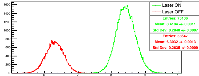
Run 4350 quartetwise, negH0: Beam ON
