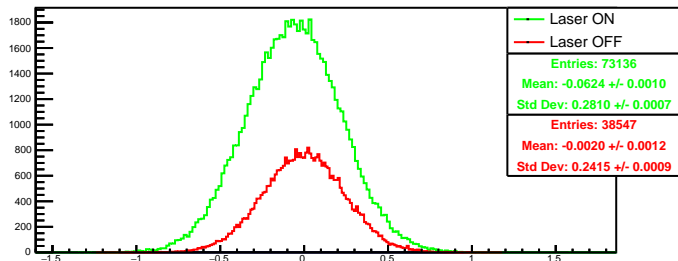
Run 4350 quartetwise, diff0: Beam ON
