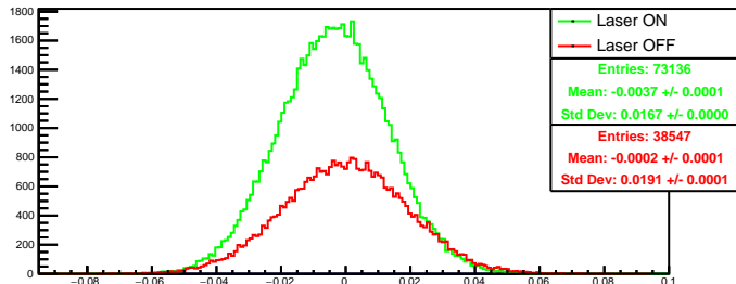
Run 4350 quartetwise, asym0: Beam ON
