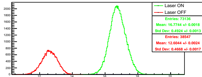
Run 4350 quartetwise, summ0: Beam ON
