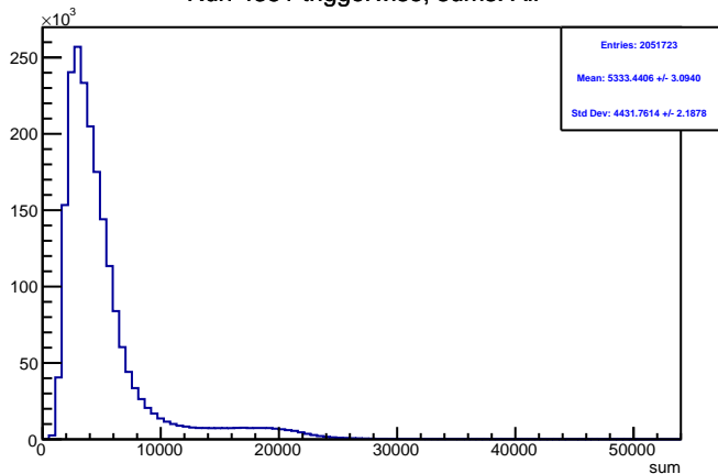
Run 4351 triggerwise, sums: All
