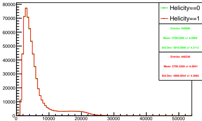
Run 4351 triggerwise, sums: Beam ON, Laser ON
