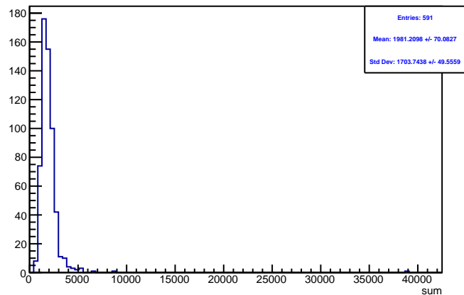
Run 4351 triggerwise, sums: Beam OFF
