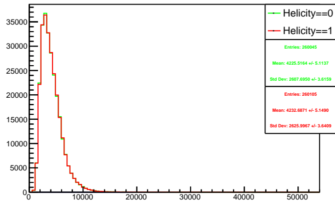
Run 4351 triggerwise, sums: Beam ON, Laser OFF
