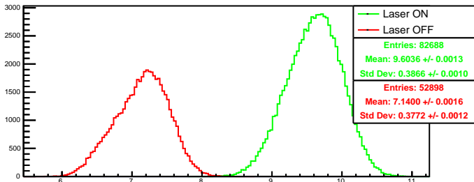
Run 4352 quartetwise, posH0: Beam ON
