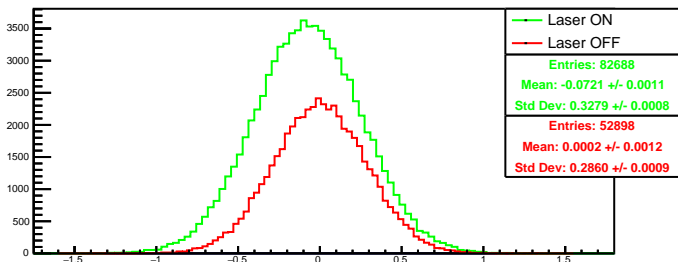
Run 4352 quartetwise, diff0: Beam ON
