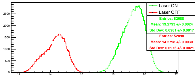
Run 4352 quartetwise, summ0: Beam ON
