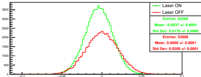
Run 4352 quartetwise, asym0: Beam ON
