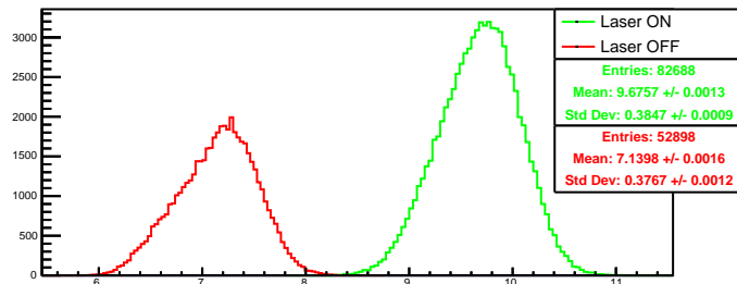
Run 4352 quartetwise, negH0: Beam ON
