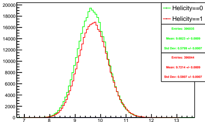
Run 4353 mpwise, acc0: Beam ON, Laser ON
