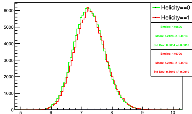
Run 4353 mpwise, acc0: Beam ON, Laser OFF
