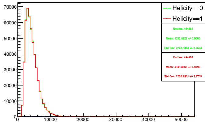
Run 4353 triggerwise, sums: Beam ON, Laser OFF
