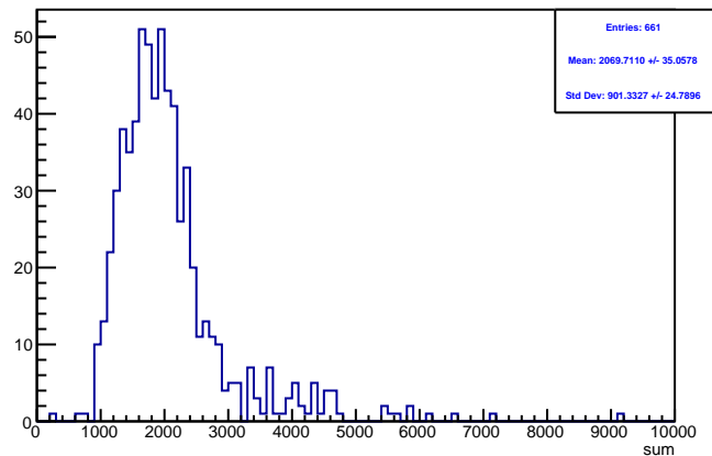
Run 4353 triggerwise, sums: Beam ON, Laser OFF
