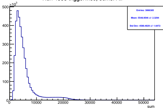
Run 4353 triggerwise, sums: All
