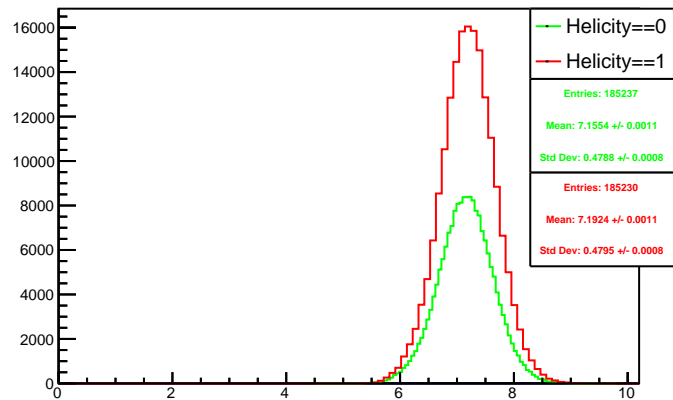
Run 4356 mpwise, acc0: Beam ON, Laser OFF
