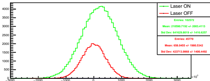
Run 4356 quartetwise, diff4: Beam ON
