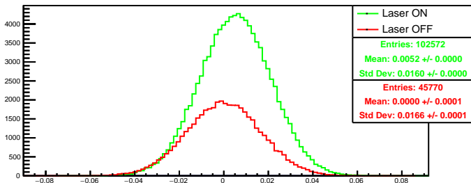
Run 4356 quartetwise, asym4: Beam ON
