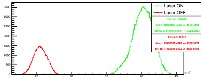
Run 4356 quartetwise, summ4: Beam ON
