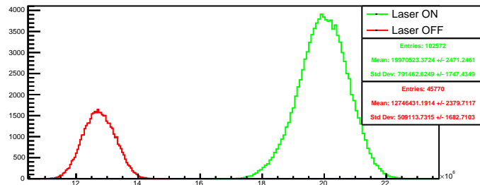
Run 4356 quartetwise, negH4: Beam ON
