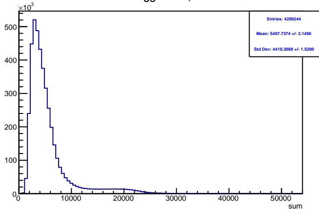
Run 4356 triggerwise, sums: All
