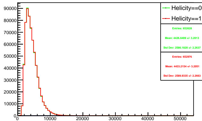
Run 4356 triggerwise, sums: Beam ON, Laser OFF
