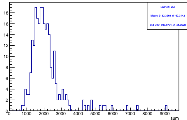
Run 4356 triggerwise, sums: Beam ON, Laser OFF
