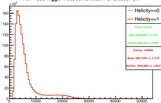
Run 4356 triggerwise, sums: Beam ON, Laser ON
