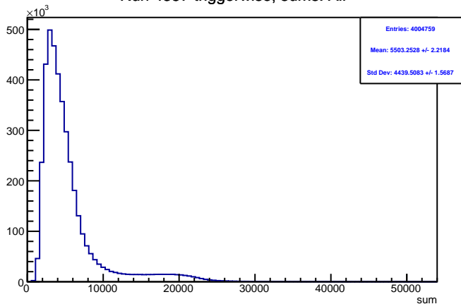
Run 4357 triggerwise, sums: All
