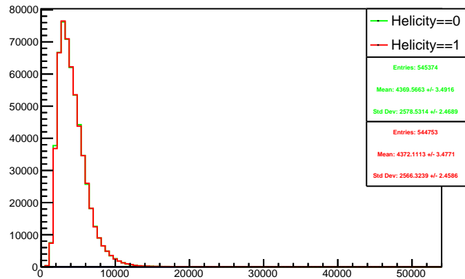
Run 4357 triggerwise, sums: Beam ON, Laser OFF
