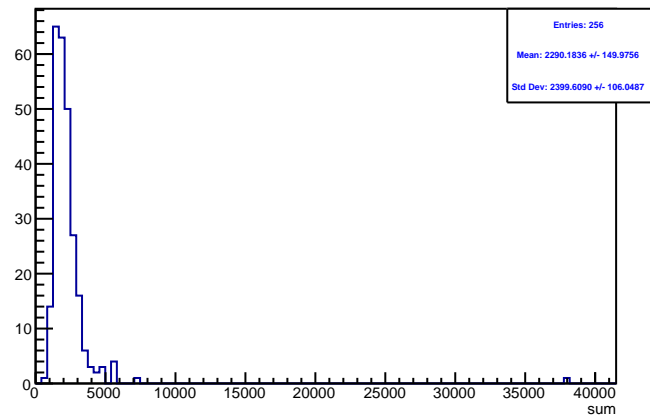
Run 4357 triggerwise, sums: Beam ON, Laser OFF
