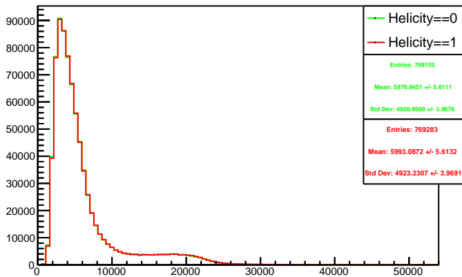
Run 4358 triggerwise, sums: Beam ON, Laser ON
