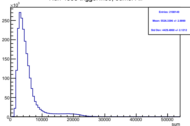
Run 4358 triggerwise, sums: All
