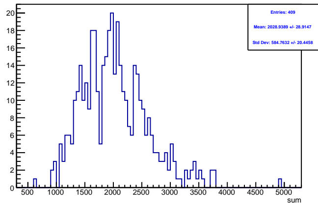
Run 4358 triggerwise, sums: Beam ON, Laser OFF
