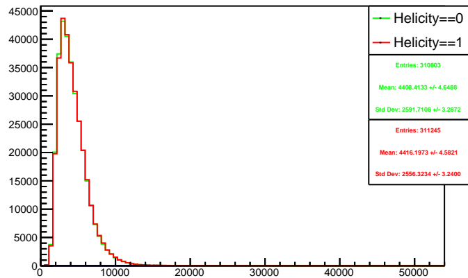
Run 4358 triggerwise, sums: Beam ON, Laser OFF
