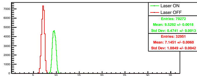
Run 4359 quartetwise, negH0: Beam ON
