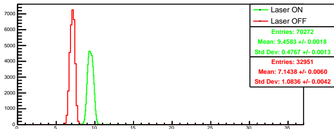
Run 4359 quartetwise, posH0: Beam ON
