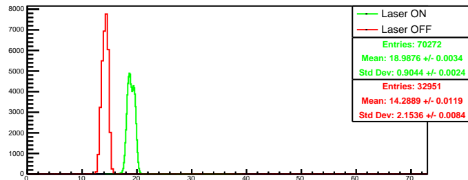
Run 4359 quartetwise, summ0: Beam ON
