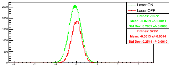
Run 4359 quartetwise, diff0: Beam ON
