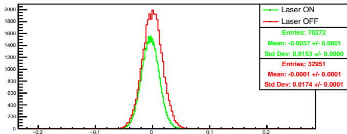
Run 4359 quartetwise, asym0: Beam ON
