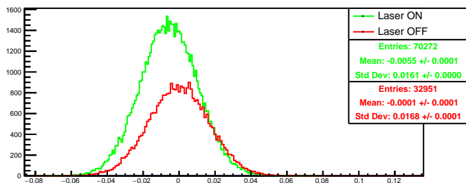
Run 4359 quartetwise, asym4: Beam ON
