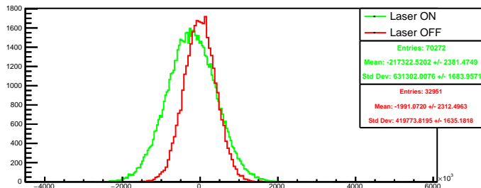
Run 4359 quartetwise, diff4: Beam ON
