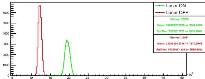
Run 4359 quartetwise, posH4: Beam ON
