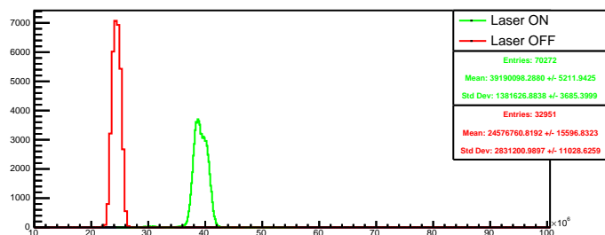
Run 4359 quartetwise, summ4: Beam ON
