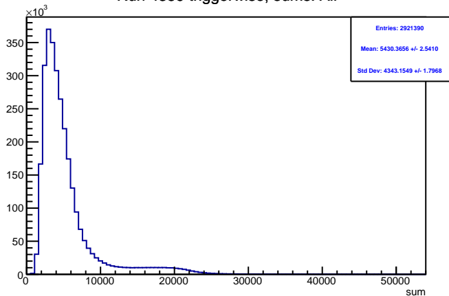
Run 4359 triggerwise, sums: All
