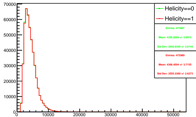
Run 4359 triggerwise, sums: Beam ON, Laser OFF
