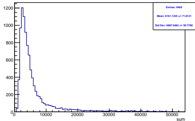
Run 4359 triggerwise, sums: Beam ON, Laser OFF
