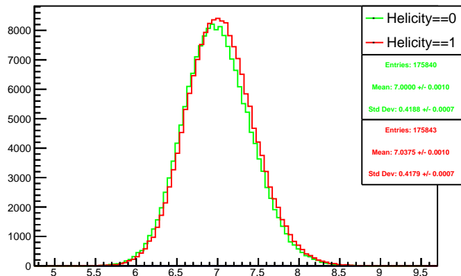
Run 4361 mpwise, acc0: Beam ON, Laser OFF
