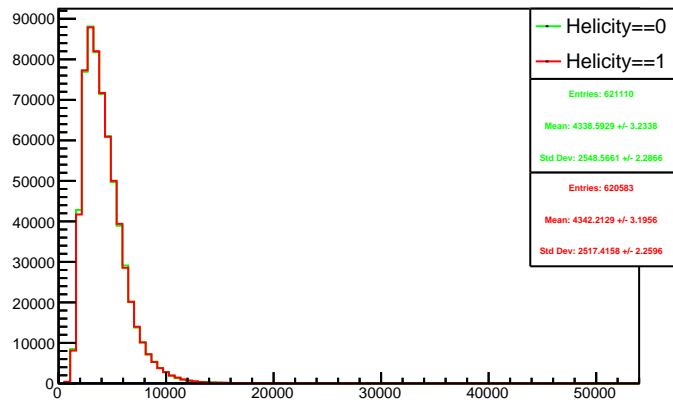
Run 4361 triggerwise, sums: Beam ON, Laser OFF
