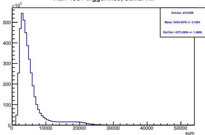
Run 4361 triggerwise, sums: All
