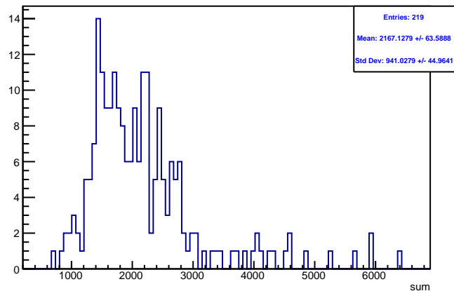
Run 4361 triggerwise, sums: Beam ON, Laser OFF
