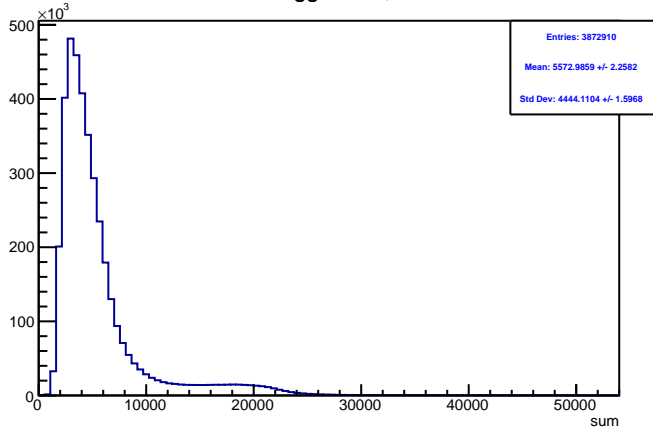
Run 4362 triggerwise, sums: All
