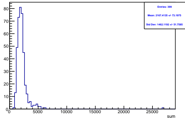
Run 4362 triggerwise, sums: Beam ON, Laser OFF
