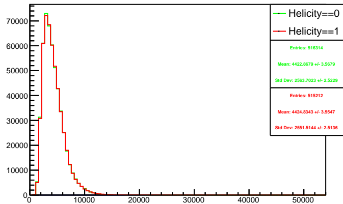
Run 4362 triggerwise, sums: Beam ON, Laser OFF
