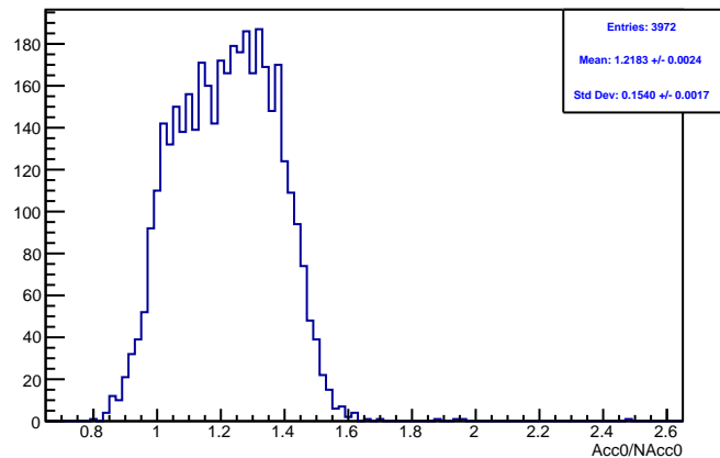
Run 4363 mpwise, acc0: Beam ON, Laser OFF
