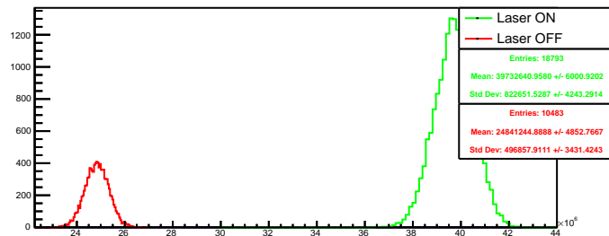
Run 4363 quartetwise, summ4: Beam ON
