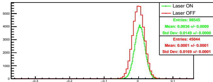
Run 4364 quartetwise, asym0: Beam ON
