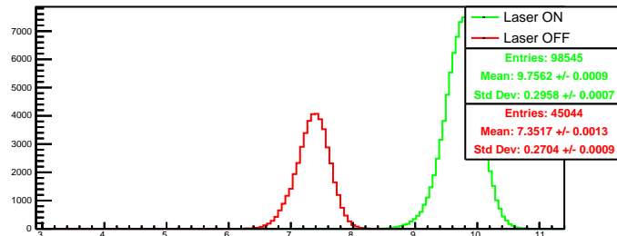
Run 4364 quartetwise, negH0: Beam ON
