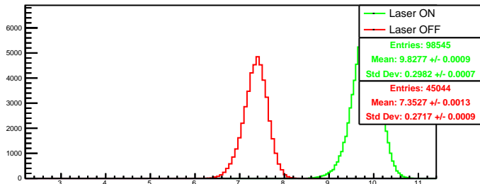
Run 4364 quartetwise, posH0: Beam ON
