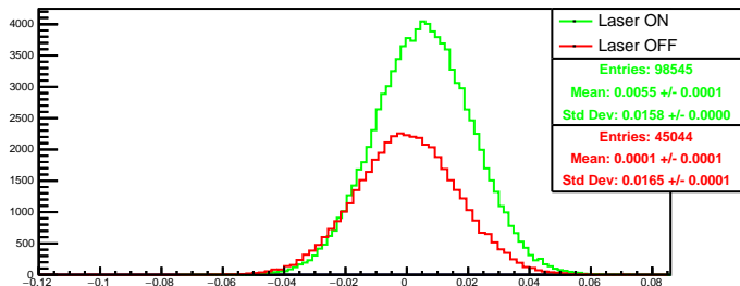
Run 4364 quartetwise, asym4: Beam ON
