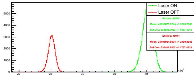
Run 4364 quartetwise, summ4: Beam ON
