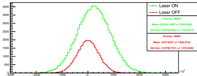
Run 4364 quartetwise, diff4: Beam ON
