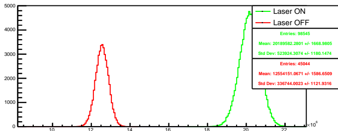
Run 4364 quartetwise, posH4: Beam ON
