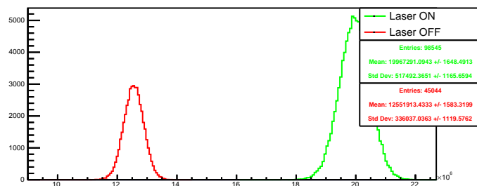
Run 4364 quartetwise, negH4: Beam ON
