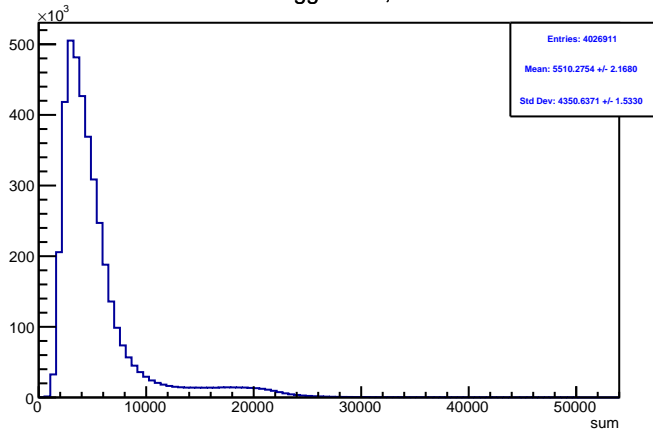
Run 4364 triggerwise, sums: All
