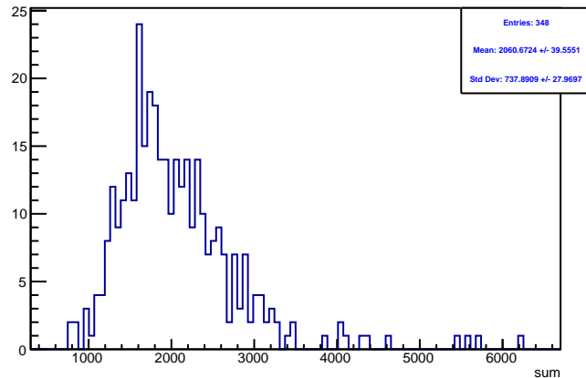
Run 4364 triggerwise, sums: Beam OFF
