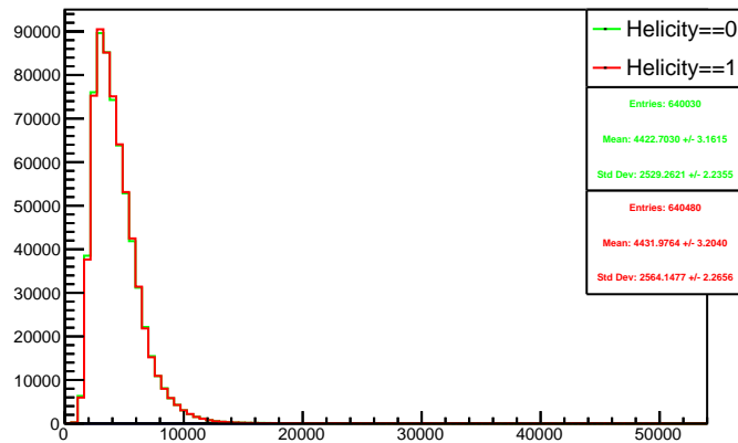
Run 4364 triggerwise, sums: Beam ON, Laser OFF
