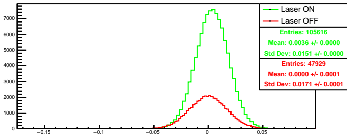
Run 4365 quartetwise, asym0: Beam ON
