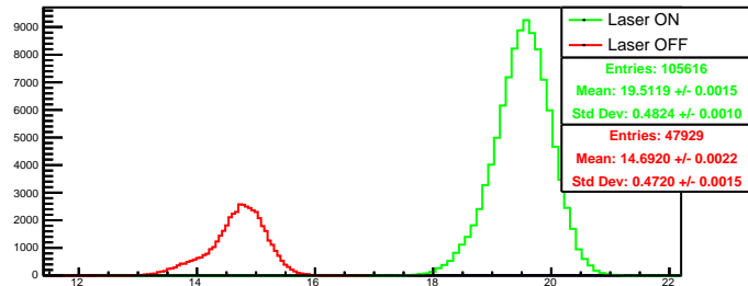
Run 4365 quartetwise, summ0: Beam ON
