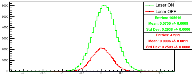
Run 4365 quartetwise, diff0: Beam ON
