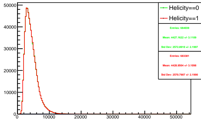
Run 4365 triggerwise, sums: Beam ON, Laser OFF
