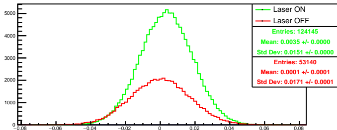
Run 4366 quartetwise, asym0: Beam ON
