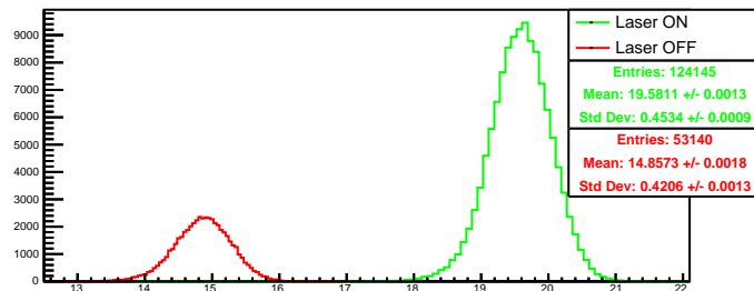
Run 4366 quartetwise, summ0: Beam ON
