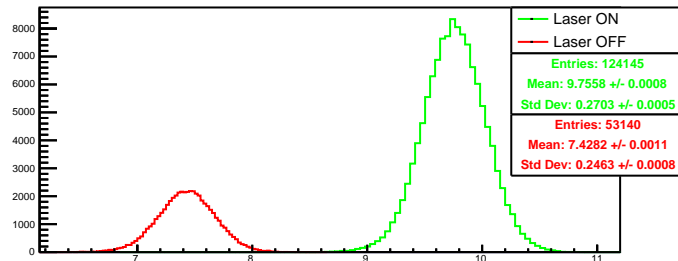
Run 4366 quartetwise, negH0: Beam ON
