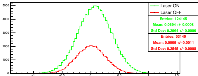
Run 4366 quartetwise, diff0: Beam ON
