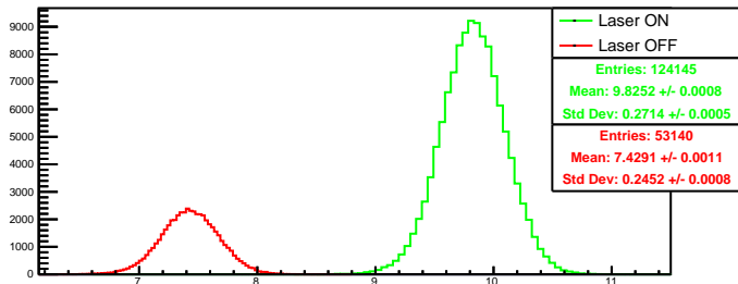
Run 4366 quartetwise, posH0: Beam ON
