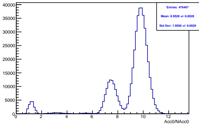
Run 4367 mpwise, acc0: Beam ON, Laser ON
