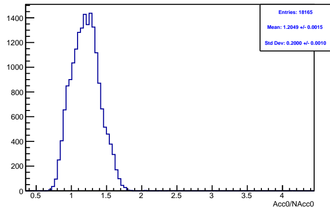
Run 4367 mpwise, acc0: Beam ON, Laser OFF
