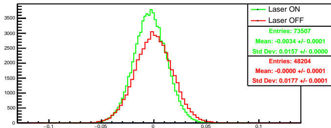
Run 4370 quartetwise, asym0: Beam ON
