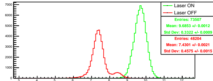
Run 4370 quartetwise, negH0: Beam ON
