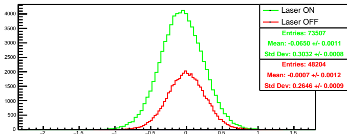
Run 4370 quartetwise, diff0: Beam ON
