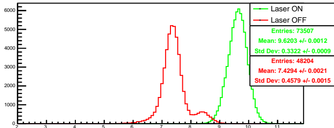
Run 4370 quartetwise, posH0: Beam ON
