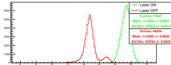
Run 4370 quartetwise, summ0: Beam ON
