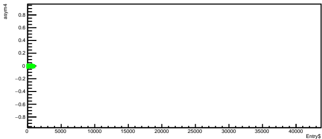
Run 4371 quartetwise, asym4 vs time
