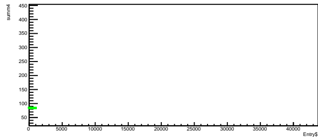
Run 4371 quartetwise, summ4 vs time
