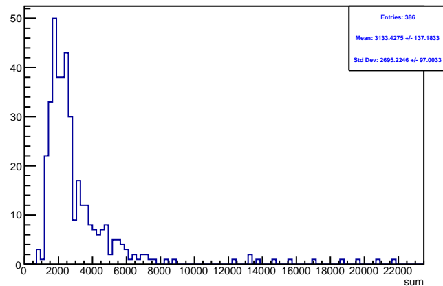
Run 4381 triggerwise, sums: Beam ON, Laser OFF
