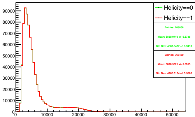
Run 4381 triggerwise, sums: Beam ON, Laser ON
