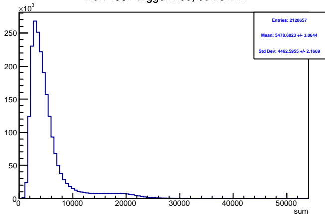
Run 4381 triggerwise, sums: All
