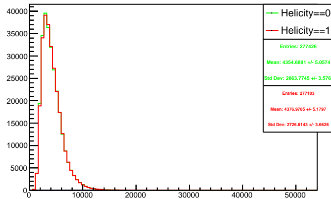
Run 4381 triggerwise, sums: Beam ON, Laser OFF
