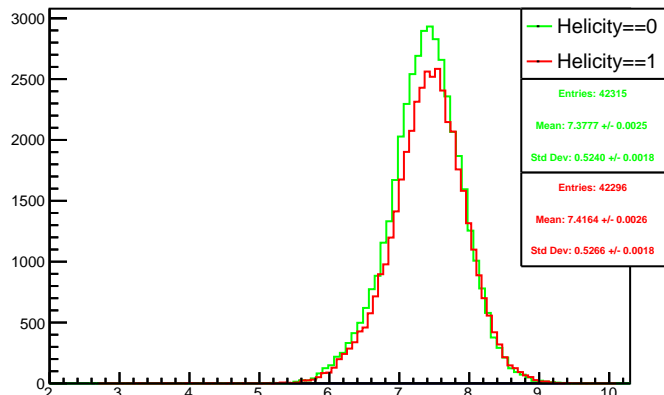
Run 4383 mpwise, acc0: Beam ON, Laser OFF
