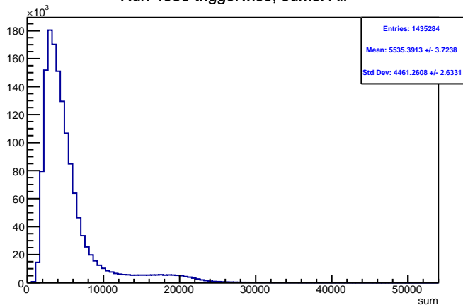
Run 4383 triggerwise, sums: All
