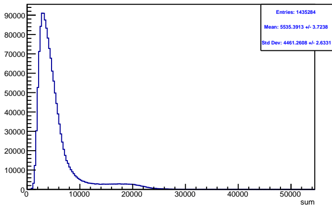
Run 4383 triggerwise, sums: Beam ON, Laser ON
