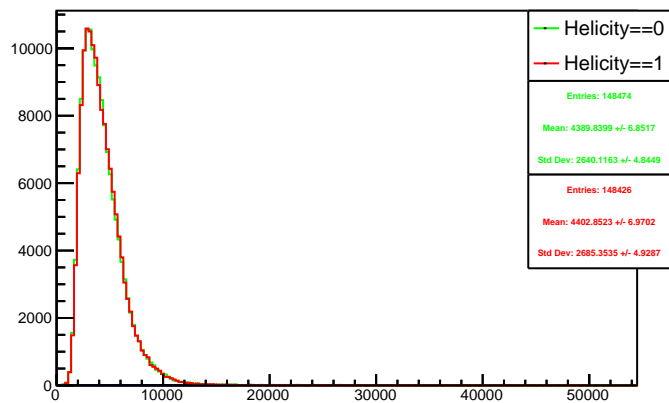
Run 4383 triggerwise, sums: Beam ON, Laser OFF
