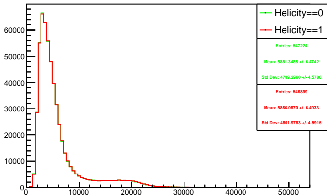
Run 4383 triggerwise, sums: Beam ON, Laser ON
