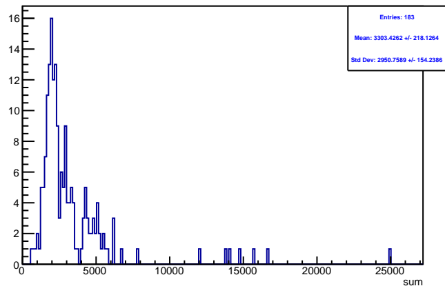
Run 4383 triggerwise, sums: Beam ON, Laser OFF
