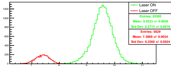
Run 4384 quartetwise, negH0: Beam ON
