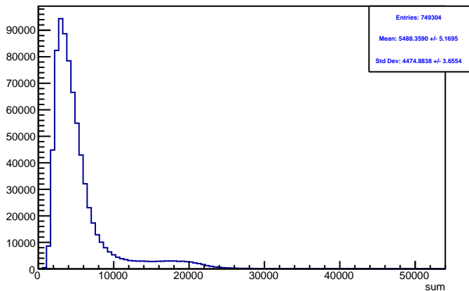
Run 4384 triggerwise, sums: All
