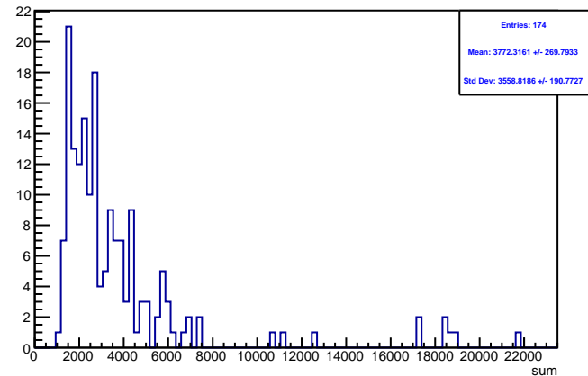
Run 4384 triggerwise, sums: Beam OFF
