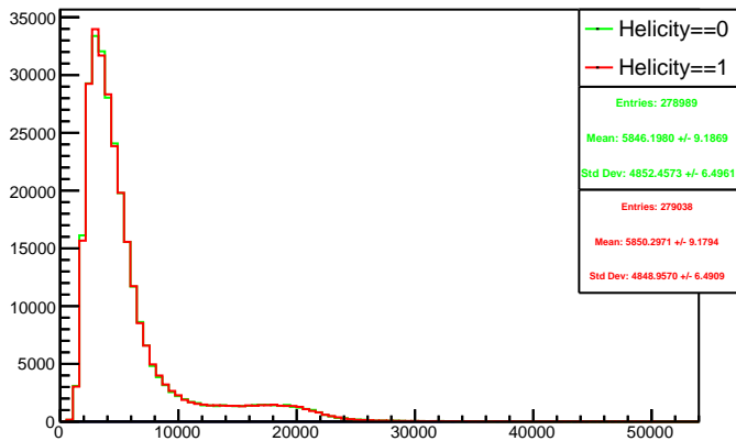
Run 4384 triggerwise, sums: Beam ON, Laser ON
