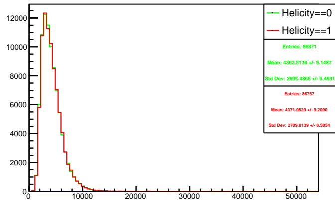
Run 4384 triggerwise, sums: Beam ON, Laser OFF
