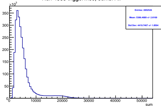
Run 4385 triggerwise, sums: All
