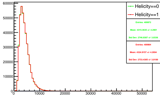
Run 4385 triggerwise, sums: Beam ON, Laser OFF
