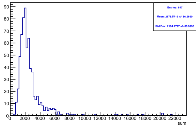
Run 4385 triggerwise, sums: Beam ON, Laser OFF
